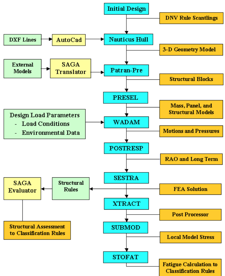
DNV Software Structural Assessment Classification Process
